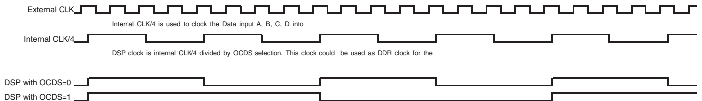
Figure 5-19. OCDS timing diagram for 4:1 MUX and IUCM1 mode
