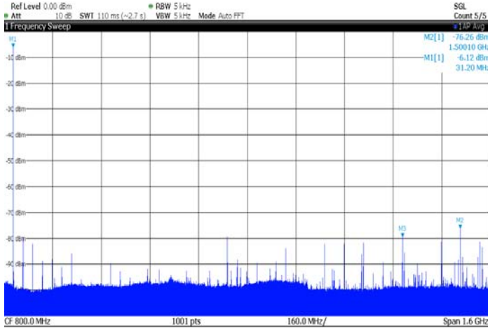
Figure 7-18. Typical SFDR spectrum in NRZ mode. F_{out} = 32\text{MHz} (1st Nyquist), MUX2:1, F_s = 3.2\text{Gps} . SFDR = 70 dBc
