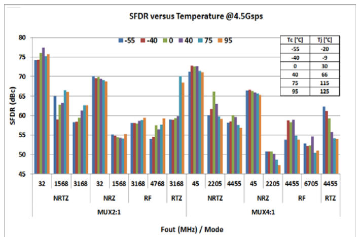
Figure 7-25. SFDR vs temperature MUX 2:1 @ 3.2 GSps MUX 4:1 @ 4.5 GSps
