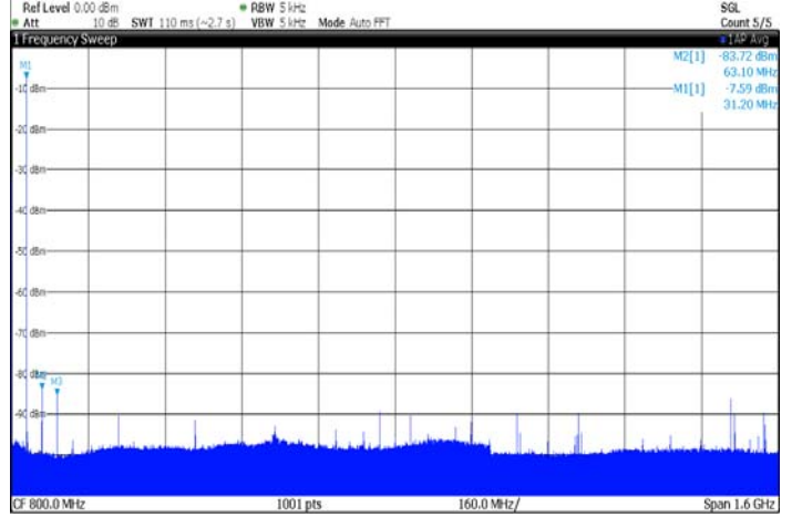
Figure 7-19. Typical SFDR spectrum in NRTZ mode. F_{out} = 32\text{MHz} (1st Nyquist), MUX2:1, F_s = 3.2\text{Gps} . SFDR = 76 dBc
