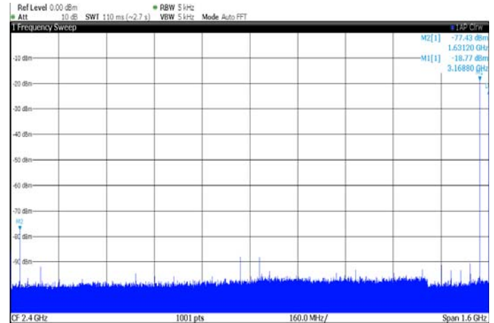
Figure 7-21. Typical SFDR spectrum in RTZ mode. F_{out} = 3168\text{MHz} (2nd Nyquist), MUX2:1, F_s = 3.2\text{Gps} . SFDR = 59 dBc
