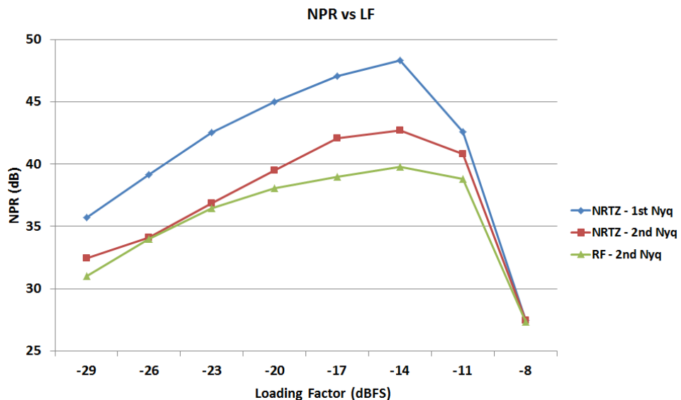
Figure 7-37. NPR versus loading factor @4.5Gbps
