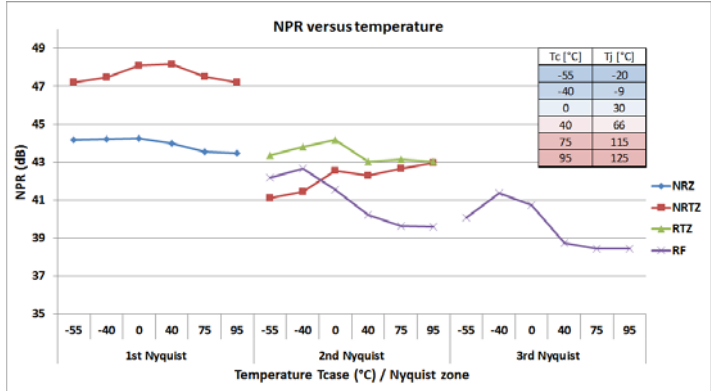
Figure 7-43. NPR versus temperature at 4.5GspS in 4:1MUX, for the four output modes from T_c = -55^{\circ}\text{C} to T_c = 95^{\circ}\text{C} ( T_j = -20^{\circ}\text{C} to 125^{\circ}\text{C} )
