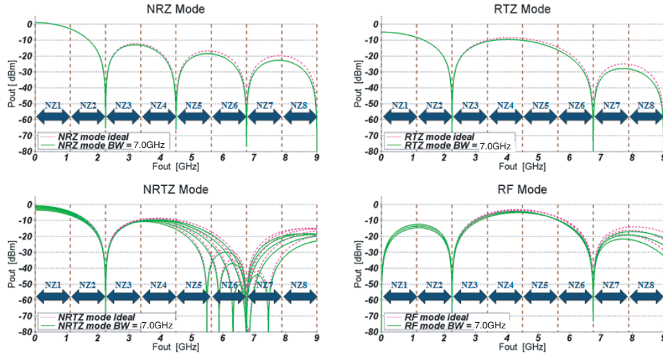
Figure 5-21. Max available Pout at nominal gain vs Fout in the four output modes at 4.5 GSps, combined with IUCM2, over eight Nyquist zones, computed for different RPW steps
