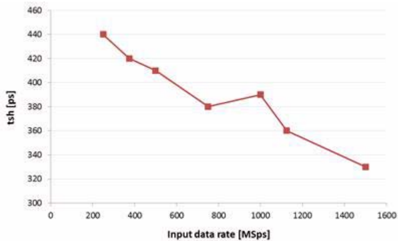
Figure 7-44. t_{SH} vs input data rate
