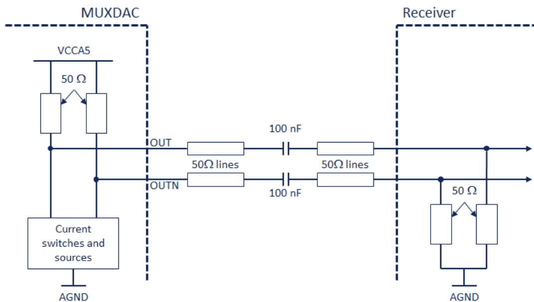
Figure 8-1. Analog output differential termination
