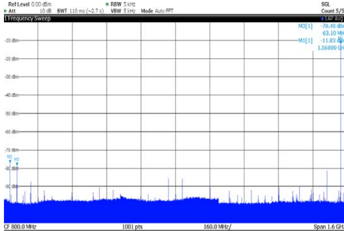
Figure 7-20. Typical SFDR spectrum in NRTZ mode. F_{out} = 1568\text{MHz} (1st Nyquist), MUX2:1, F_s = 3.2\text{Gps} . SFDR = 65 dBc
